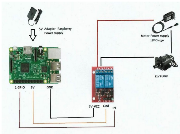
Figure 1- Circuit Diagram-Plant Pulse
