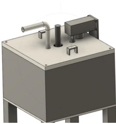
Figure 7: - Inlet of oil and actuator
