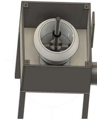
Figure 5: - Housing and coupling done inside the centrifugal pot
